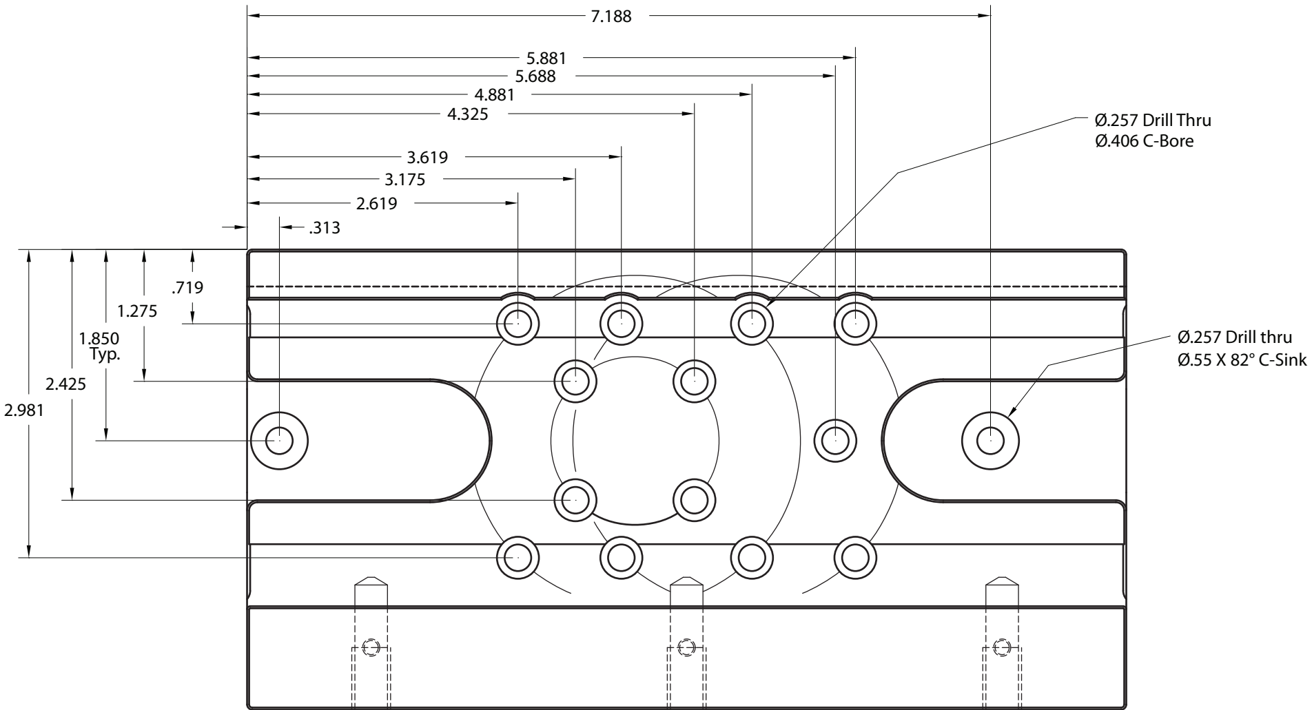
8.5" Dovetail Saddle (DOVELM2)
