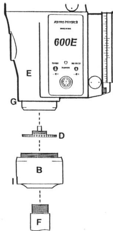
600E Mount Dec. Encoder Assembly
